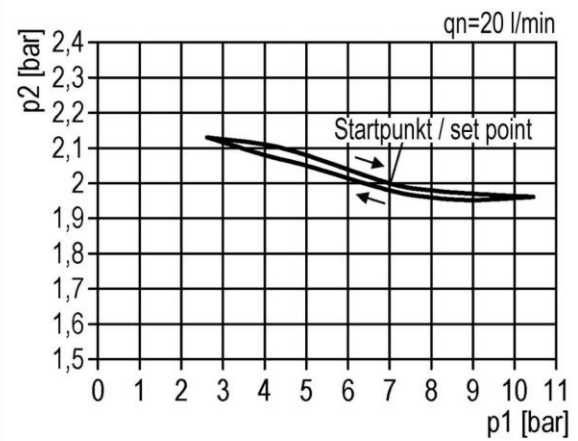
pressure characteristic
